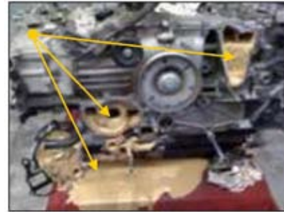
This mess was in every part of the cooling system and resulted in a complete system disassembly. The heater core and radiator had to be replaced.
