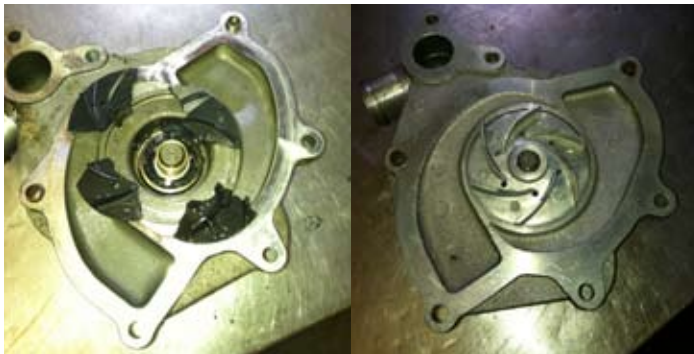
Pump with plastic impeller
