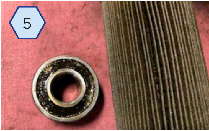
You can see debris from this old bearing coming apart. Fortunately, the filter shows no large pieces in it.
